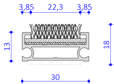
Detail with inlay needlepunch
