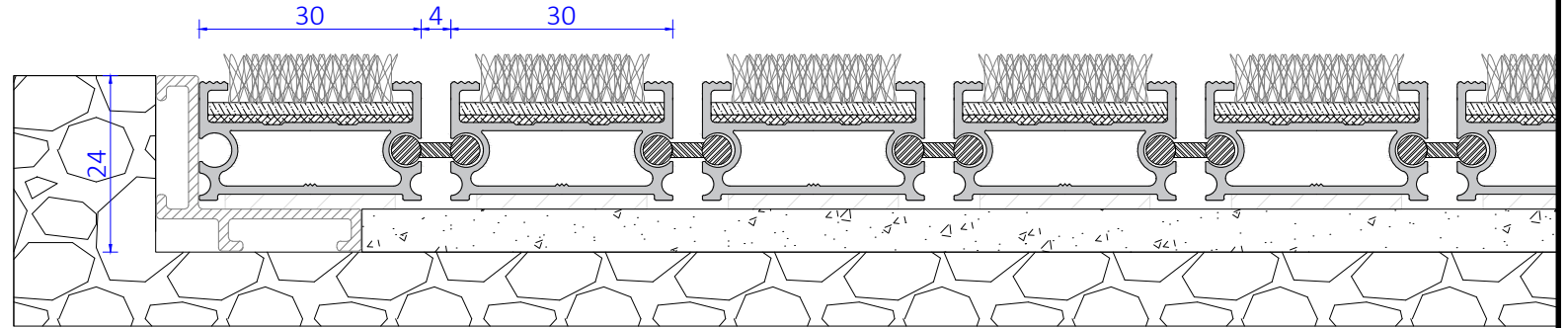
Vertical cross section mat
