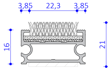
Detail with inlay needlepunch
